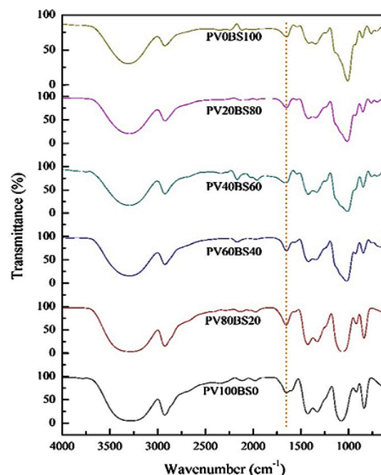
Fig. 3: FTIR spectrum of all samples tested
