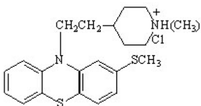
Scheme 1: Thioridazine-HCl (TRH)
