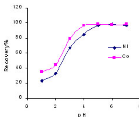
Fig. -1: Effect of pH on the recovery of cobalt and nickel. (Sample solution: 250 ml of solution containing 0.5 µg of each metal at 25 ml min -1 flow rate. Eluent: 10 ml of 0.01 M of nitric acid solution at 7 ml min -1 flow rate. Amount of ligand: 10 mg).
