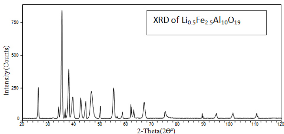
Fig. 1: X-ray diffraction of \text{Li}_{0.5}\text{Fe}_{2.5}\text{Al}_{10}\text{O}_{19}
