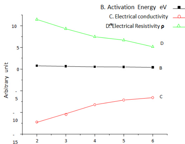
Fig. 2: Composition of Al Ions in Lithium ferrites \text{Li}_{0.5}\text{Fe}_{0.5+x}\text{Al}_{12-x}\text{O}_{19} ( x=2,3,4,5,6 )
