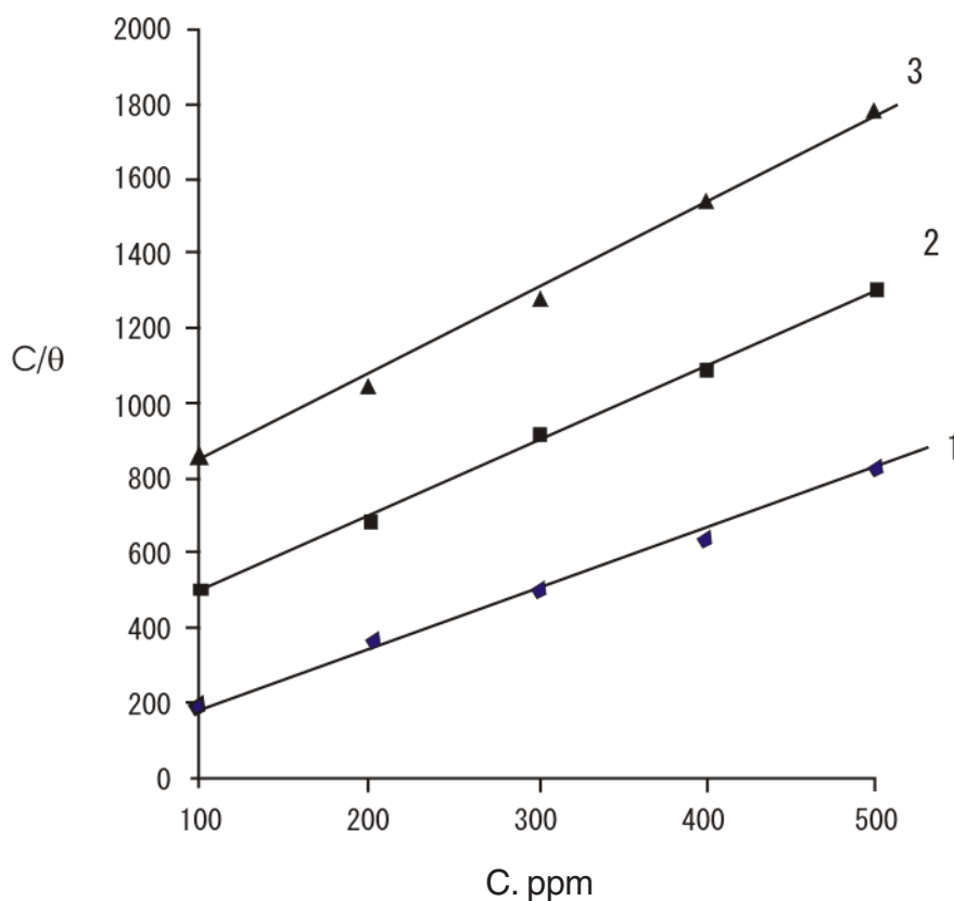
Fig. - 2: Langmuir adsorption isotherm 1) compound I 2) compound II 3) compound III
