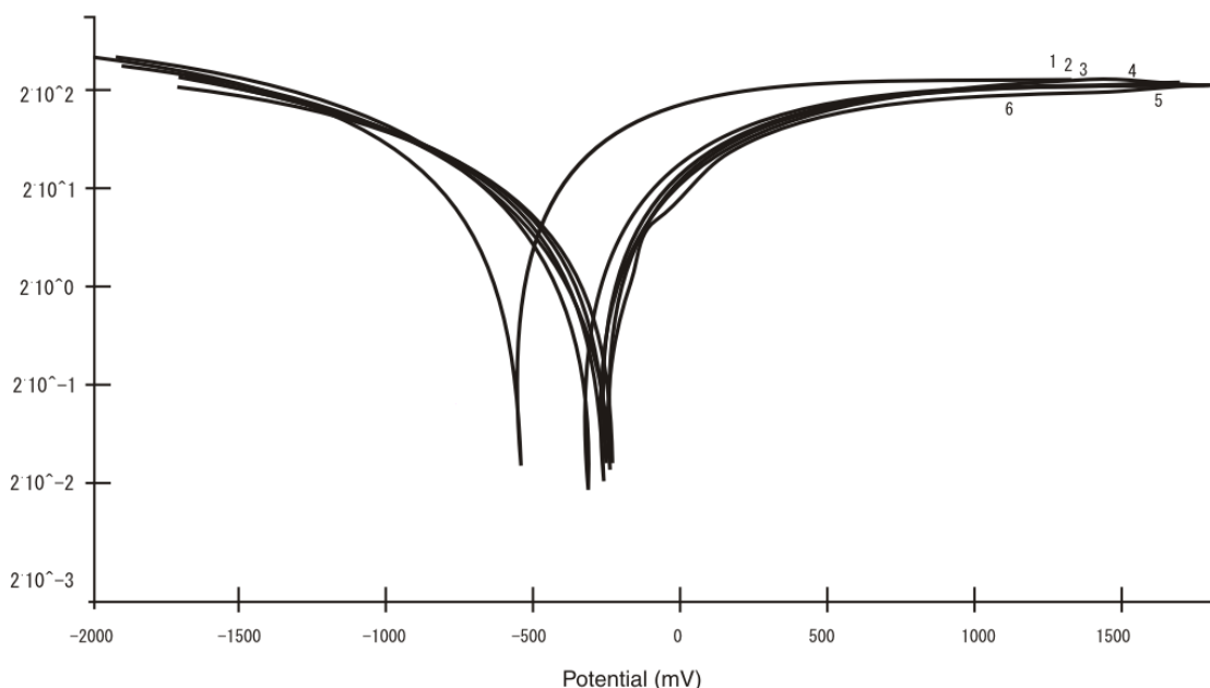
Fig. - 1: Galvanostatic polarization curves for iron electrode in 1M HCl in absence and presence of different concentration of compound III 1) 0.00ppm 2) 100 ppm 3) 200 ppm 4) 300 ppm 5) 400 ppm 6) 500 ppm.
